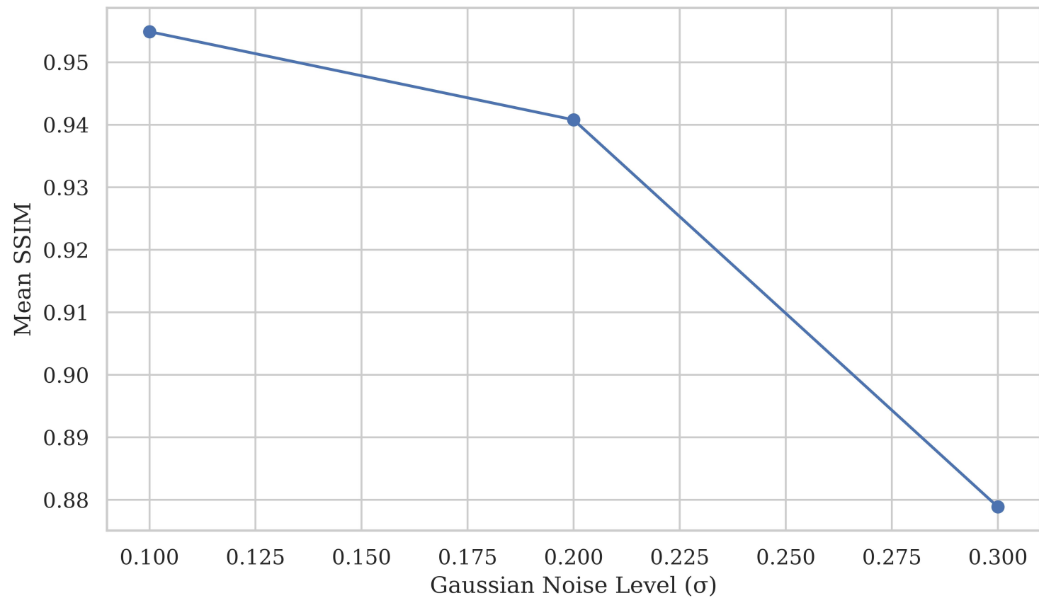
Noise Level vs SSIM
